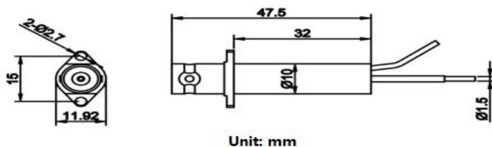
(CSD005, CSD01, CSD02 机械规格)
